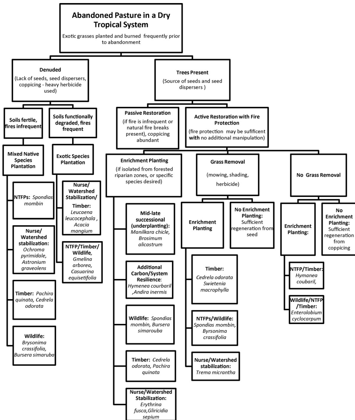
Fig. 3. Restoration pathways of dry tropical forests for different biological and social circumstances. The assumption is that abandoned pastures have been historically grazed by cattle and burned frequently. See Table 2 for rationale of selected tree species.
