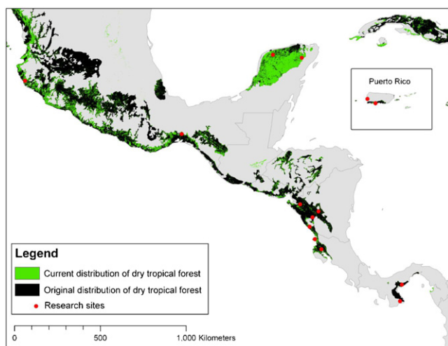
Fig. 1. The original distribution of dry tropical forests was derived from WWF ecoregion dataset (Olson et al., 2001), combining two ecoregions: tropical and subtropical dry broadleaf forests and tropical and subtropical grasslands, savannas, and shrublands. The current distribution was acquired from Miles et al. (2006). For further information, email: spatialanalysis@unep-wcmc.org . They determined this current distribution from the WWF ecoregion data, overlaid with the MODIS (Moderate Resolution Imaging Spectroradiometer) dataset, identifying areas with at least 40% forest cover. Locations of current experimental and observational research in abandoned pastures, plantations, and secondary forests are shown in red.
