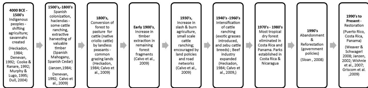
Fig. 2. Timeline of deforestation and degradation within dry tropical forests in Central America (Costa Rica and Panama).
